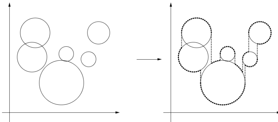
Figure 2.1: Extending an open set into an open strip
