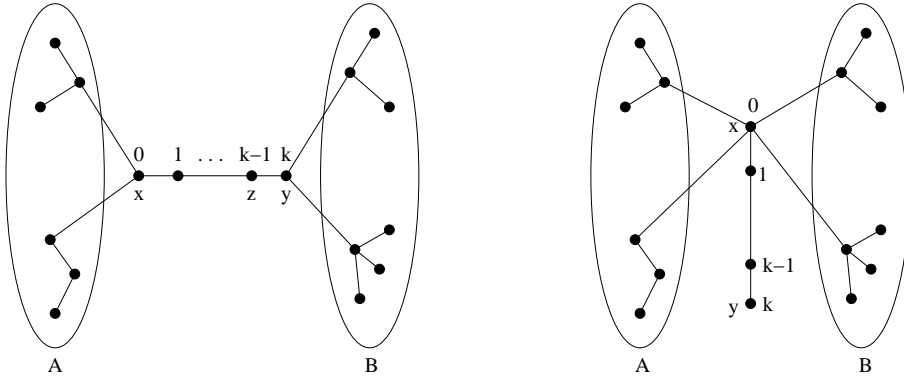
FIGURE 3. The KC-transformation.
