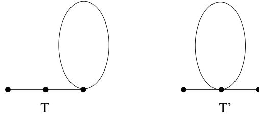
FIGURE 6. Short-path shift.
