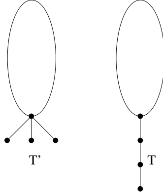
FIGURE 7. Claw-deletion.
