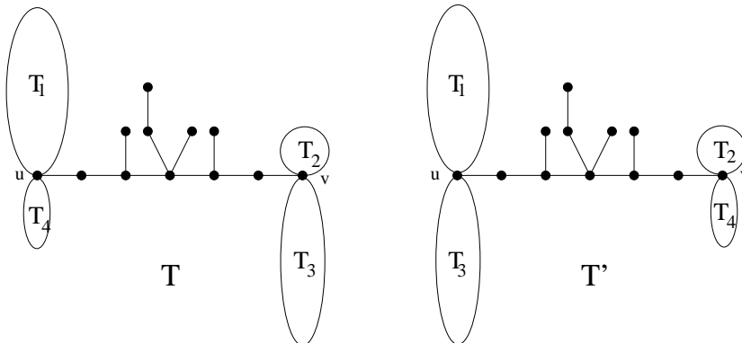
FIGURE 5. LS-switch.
