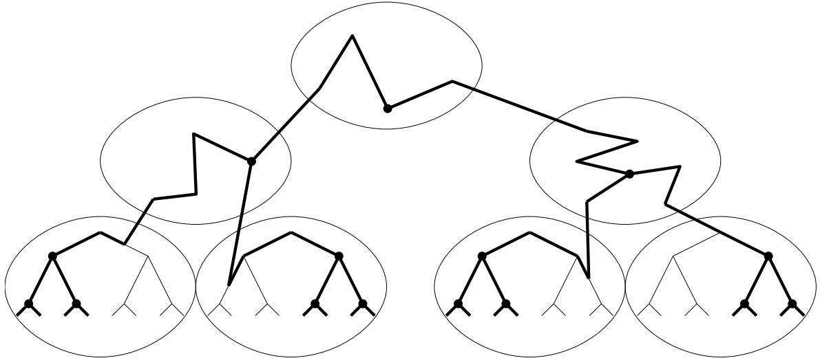
Figure 1: Constructing big binary trees using induction for structure trees.
