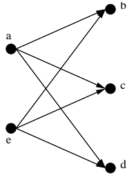
FIG. 4.1. The largest sink-stable set in this graph is S = \{b, c, d\} . An optimal covering consists of a circuit C = \{ab, be, ec, ca\} and an edge ad , the total value of this covering is 3.
