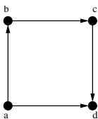
FIG. 1.1. Every node is a sink-stable set of size 1, while the stable set \{a, c\} is not sink-stable.
